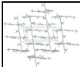
Fig. 2. The molecular packing for C 36 H 40 ClN 6 Ni 2 O 9 viewed down the b axis showing the linear chains of bis(4-methoxysalicyldene)ethylenediaminomanganese(III) moieties bridged by acetate groups and methanol solvate hydrogen bonded to the phenolic oxygen atoms (shown by dashed lines).
